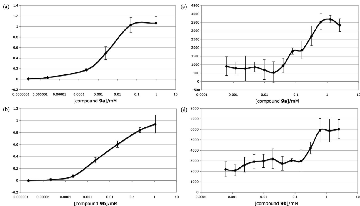
Figure 2. a) and b) Binding of avidin-HRP to the immobilized model compounds 9a and 9b . c) and d) binding of avidin-FITC to the immobilized model compounds 9a and 9b . The compounds were serially diluted and covalently immobilized in wells of clear (a and b) or white (c and d) aminofunctionalized microtiter plates and probed with the given avidin conjugate. The concentrations of the model compounds added to the well are given on the x-axis. The points represent the average of triplicate runs and error bars are set to \pm one standard deviation. In the graphs, the average value of a triplicate of controls was subtracted from the observed values (triplicates).
