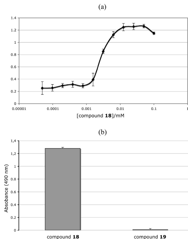
Figure 4. a) Binding of galactose selective lectin from Ricinus communis (RCA 120 ) to the immobilized neoglycolipid 18 . The compound was serially diluted in the wells and covalently immobilized to the amino-functionalized wells. The immobilized neoglycolipid was detected with biotin-conjugated RCA 120 and avidin-HRP. The concentration of the neoglycolipid added to the well is given on the x axis. The points represent the average of triplicate runs and error bars are set to \pm one standard deviation. In the graphs, the average value of a triplicate of controls was subtracted from the observed absorbencies (triplicates). b) Binding of the galactose selective lectin RCA 120 to the immobilized neoglycolipids 18 and 19 (0.025 mM). The average value of a triplicate of controls was subtracted from the observed absorbencies (triplicates). No binding of the lectin was observed in the wells reacted with the glucose neoglycolipid 19 .
