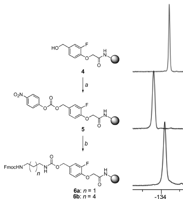
Scheme 1. Synthesis of the carbamate resin 6a and 6b and gel-phase 19 F NMR spectra recorded for resin 4 , 5 , and 6b . a) N -methyl morpholine, p -nitrophenyl chloroformate, CH 2 Cl 2 ; b) N -Fmoc-1,3-diaminopropane hydrochloride or N -Fmoc-1,6-diaminohexane hydrochloride, N,N' -diisopropylethylamine, DMF.
