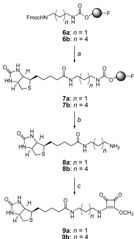
Scheme 2. Synthesis of model compounds 9a and 9b . a) i) Piperidine (20% in DMF); ii) HOAt, DIC, D-biotin, DMF; b) 3 \times TFA (90% in H 2 O), quantitative yield and 70% yield, respectively; c) dimethyl squarate, TEA, DMF, quantitative yield for both 9a and 9b .
