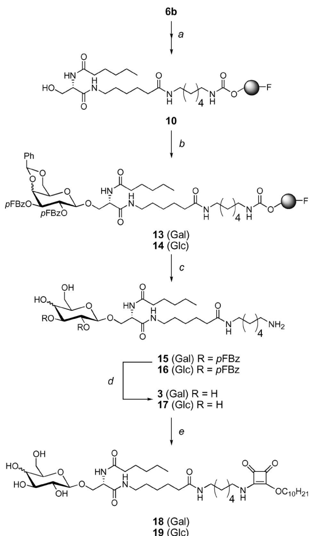
Scheme 3. Synthesis of squaric amide ester neoglycolipid 18 and 19 . a a) i) Piperidine (20% in DMF); ii) Fmoc-6-amino-hexanoic acid, HOBT, DIC, DMF, BFB; iii) Piperidine (20% in DMF); iv) Fmoc-L-serine HOBT, DIC, DMF, BFB; v) piperidine (20% in DMF); vi) hexanoic acid, HOBT, DIC, DMF, BFB; b) 11 or 12 , QOTf, NBS, MS 3 Å, CH 2 Cl 2 , 65% and 57% respectively; c) TFA/H 2 O, 9:1, 24% and 12% yield respectively; d) NaOMe (0.20 M in MeOH), MeOH; e) didecyl squarate, TEA, DMF, 20% and 27% yield respectively.
