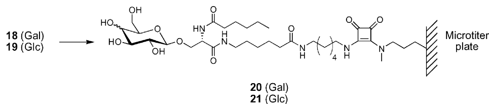
Scheme 4. Immobilization of squaric amide ester neoglycolipid 18 and 19 in amino-functionalized microtiter plates. a) NaHCO 3 buffer (pH 9), CovaLink™ (Nunc A/S, Denmark) microtiter plate.
