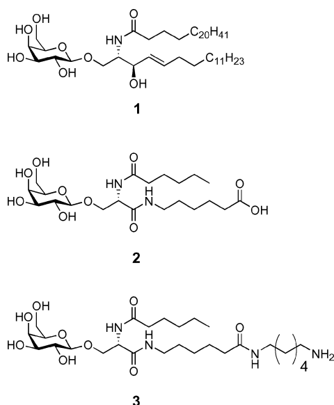
Figure 1. \beta -Galactosylceramide 1 and the serine-based analogs 2 and 3 .
